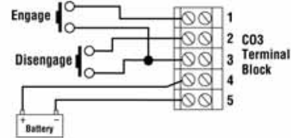
Figure 3: Customer Wiring
