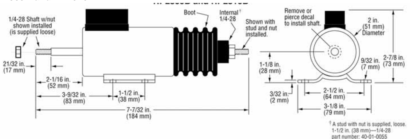
Solenoid Shown with Plunger Seated (Coil Energized)
